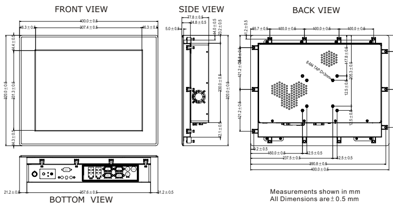
IP65 Front
